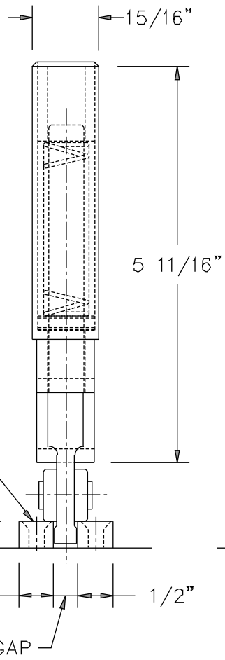
0739.00026 FLOOR GUIDE 0739.00028 FLOOR GUIDE TRACK - 10' LENGTHS STANDARD
