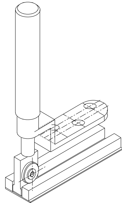
0739.00026 FLOOR GUIDE 0739.00028 FLOOR GUIDE TRACK - 10' LENGTHS STANDARD
