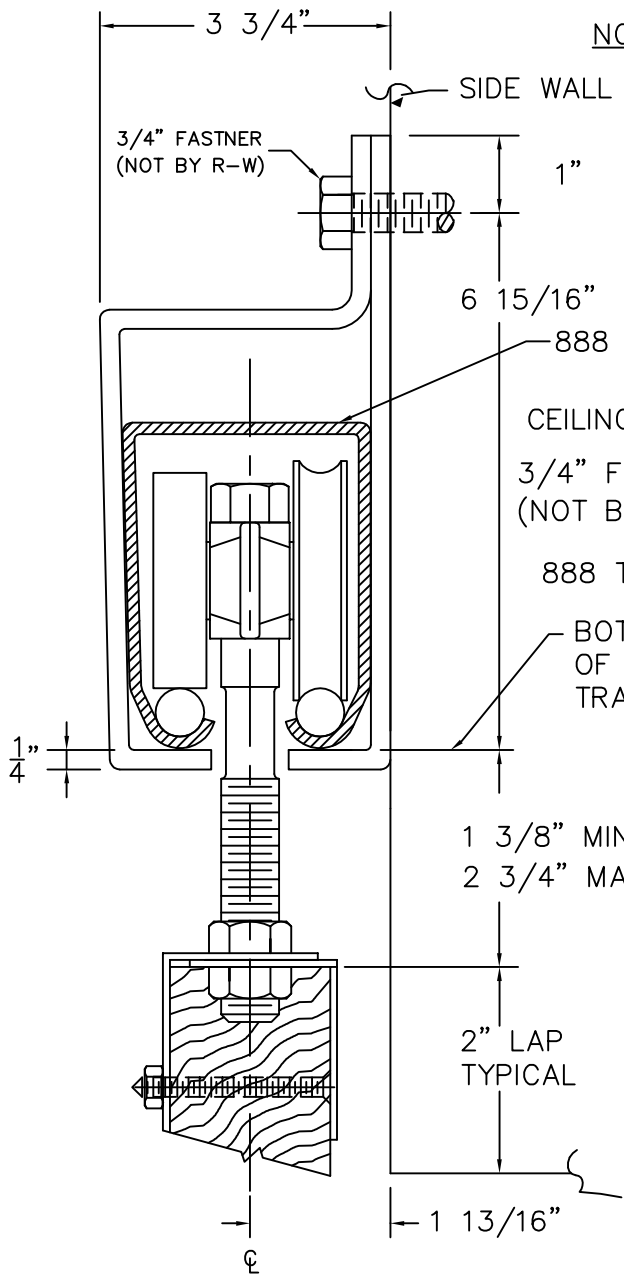
STANDARD HEAD SECTION USING HANGERS AND SIDE WALL BRACKETS
